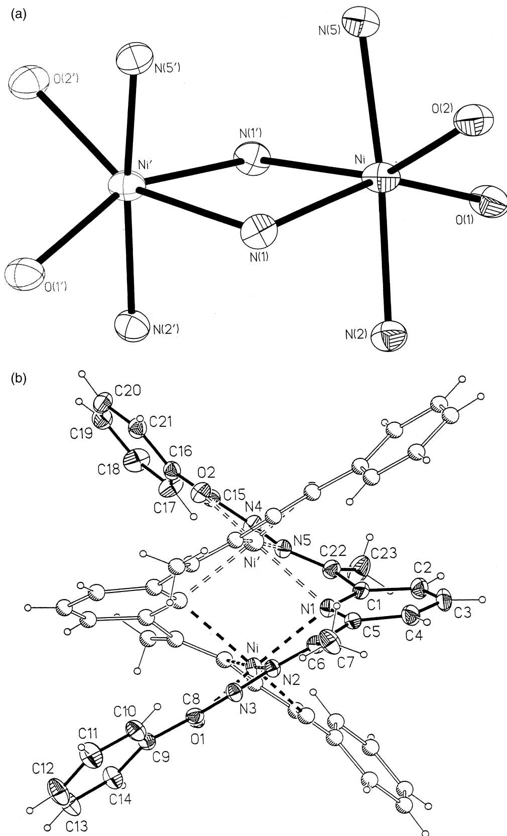
Figure 3. (a) View of the coordination polyhedron around the two equivalent nickel atoms related by the symmetry operation 1/2-x, y, -z . Thermal ellipsoids are drawn at 30% level. (b) View of the dimer along the crystallographic two-fold axis showing the numbering Scheme of the asymmetric unit. The bridging N-bonds are represented by shaded lines. Thermal ellipsoids are drawn at 30% level while hydrogen and equivalent atom size is arbitrary.
