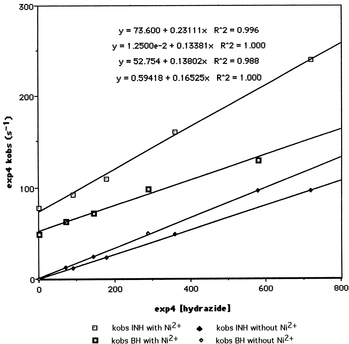
Figure 2. Plots of k_{\text{obs}} ( \text{s}^{-1} ) versus hydrazide concentration for the condensation of dap and hydrazide in the presence and in the absence of \text{Ni}^{2+} .
