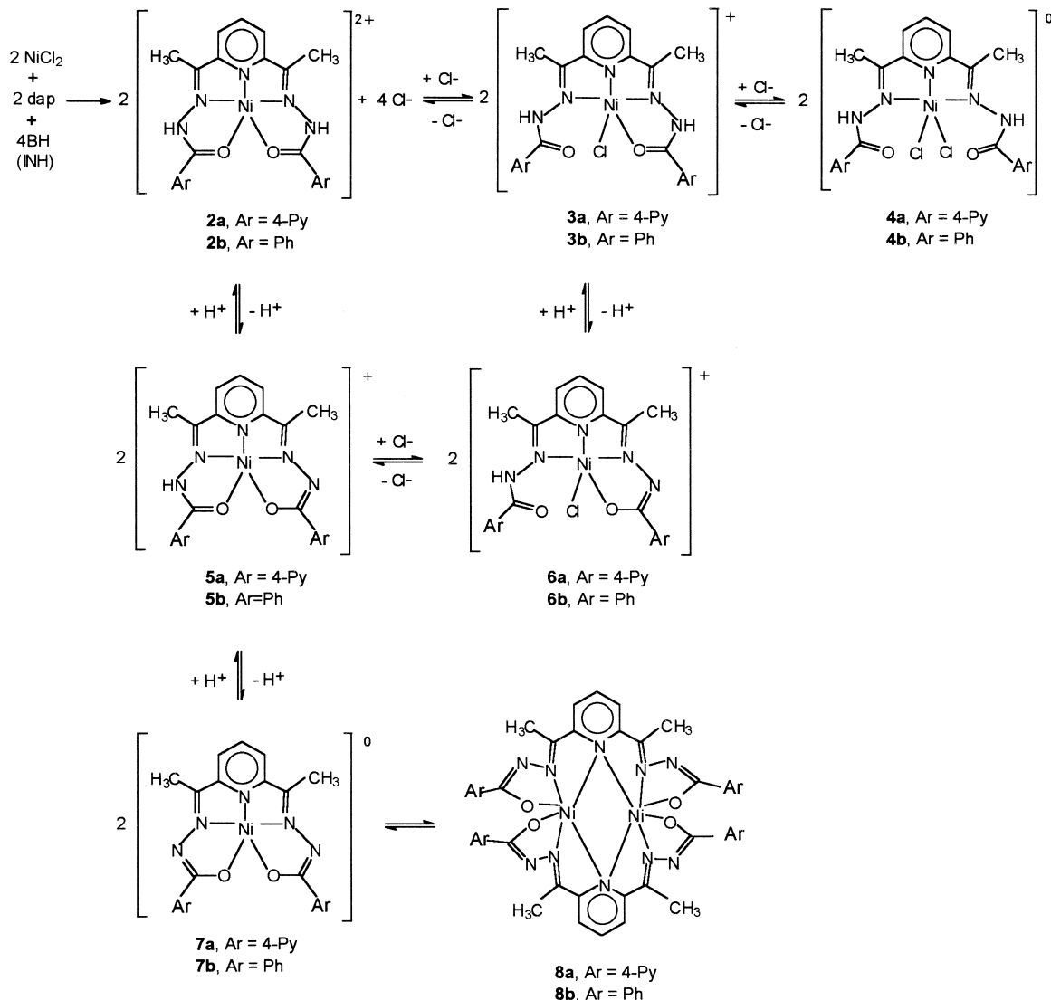
Scheme 1. For simplicity the coordinated molecules of solvent have not been reported in the Scheme.
