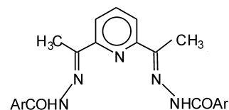
1a , Ar=Py ( \text{H}_2\text{dapin} )
